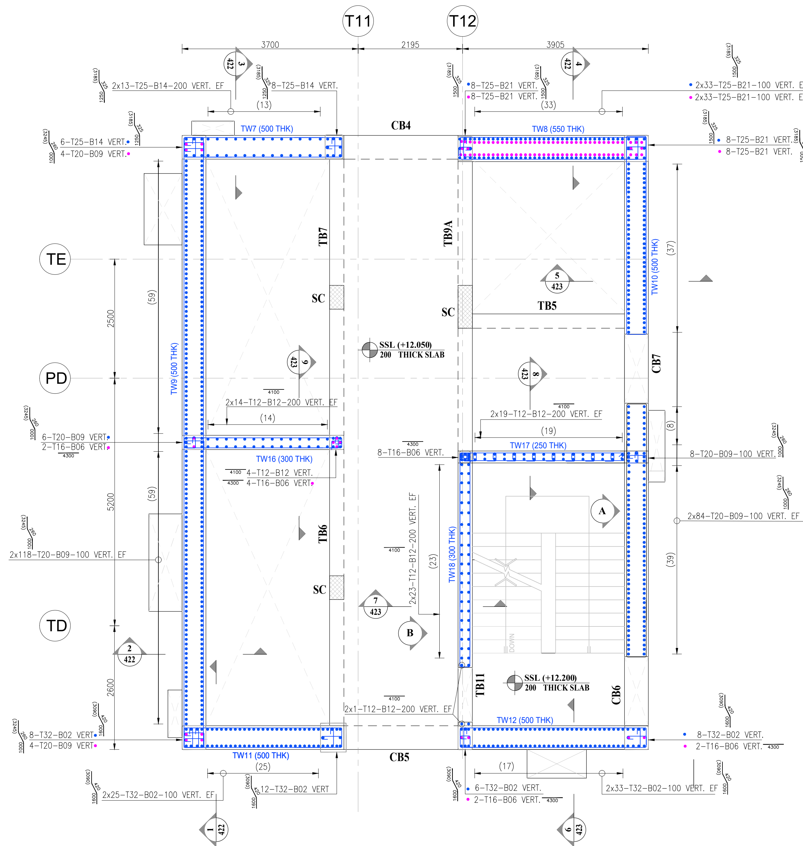
DETAIL-A TOWER CORE WALL VERTICAL REINFORCEMENT DETAILS
