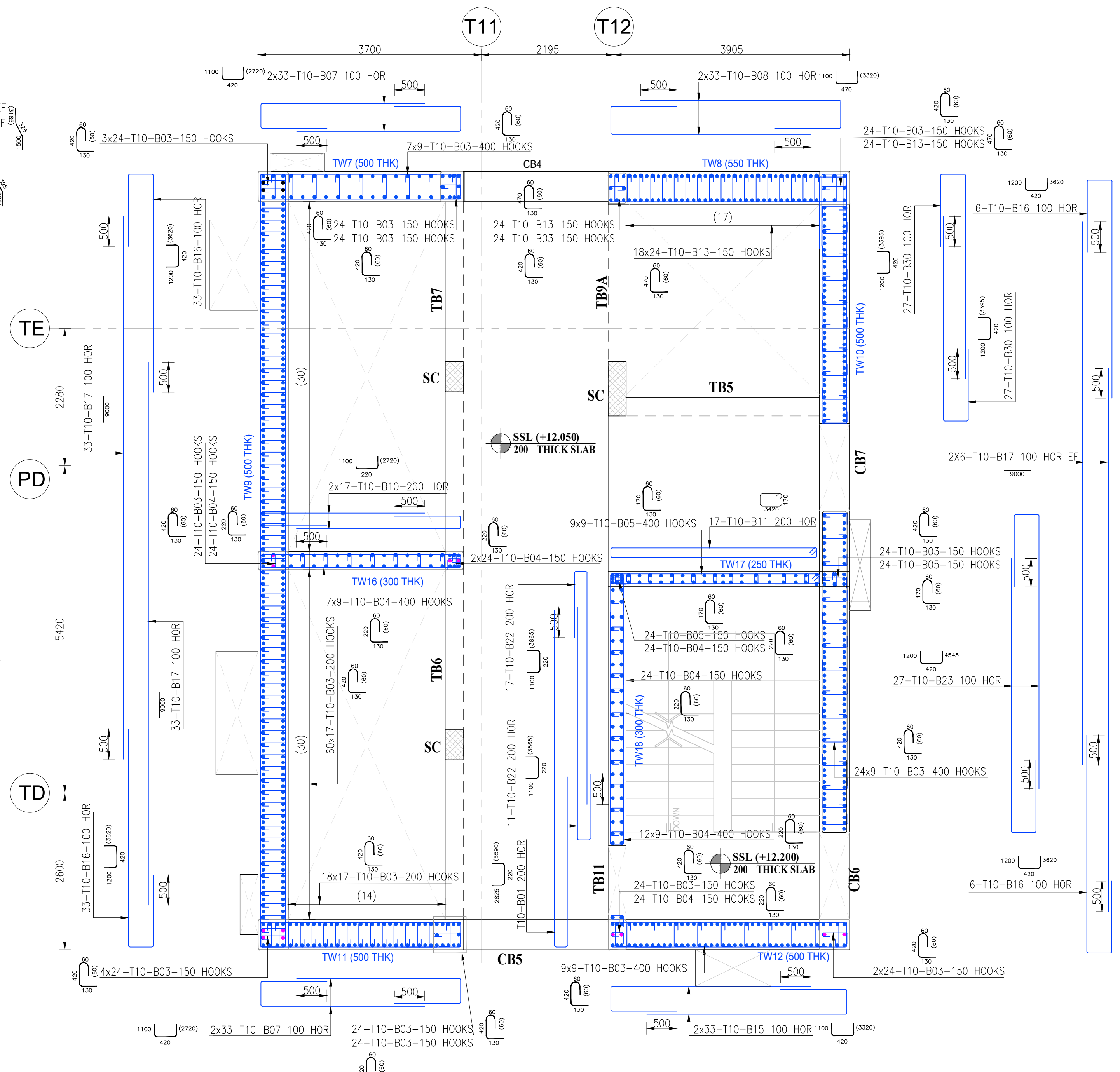
DETAIL-A TOWER CORE WALL HORIZONTAL REINFORCEMENT DETAILS
